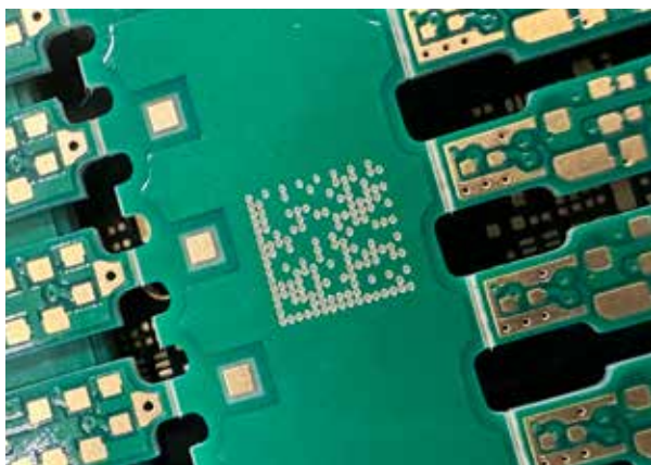
PCB marking
